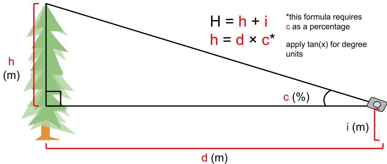
Figure 5. Clinometer methodology.
